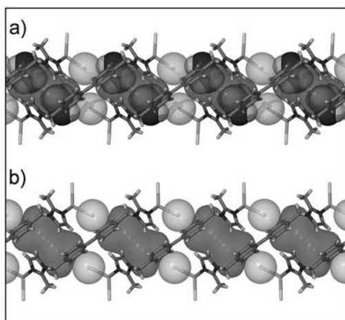
Figure 1. Columnar stacking of 1 along [001] (horizontal direction) as viewed down [010]. Each guest-accessible cavity (semi-transparent surface) is defined by four metallocycles and has an approximately rectangular cross-section terminated by a chloride ion (semi-transparent sphere) at each of the short ends. a) Each cavity (123 Å 3 ) in the structure of 1 ·2 MeOH is occupied by a pair of methanol molecules. b) Upon desolvation at room temperature the crystals remain intact and the cavities maintain their shape (117 Å 3 ).
